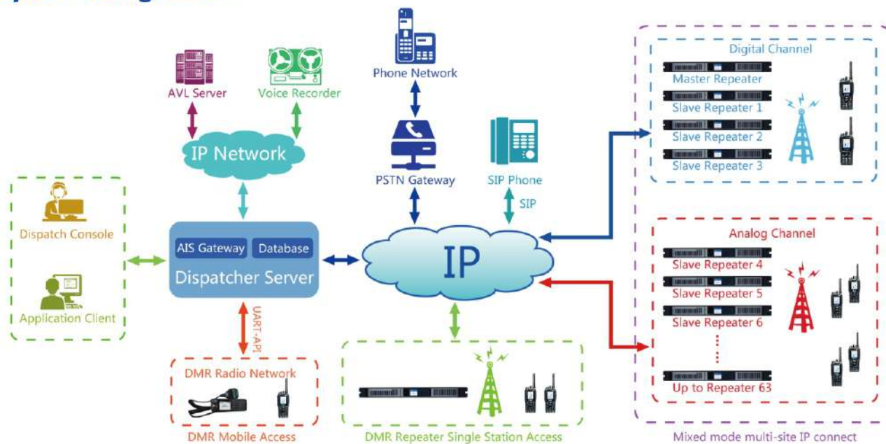
Mixed analog & digital DMR conventional system
